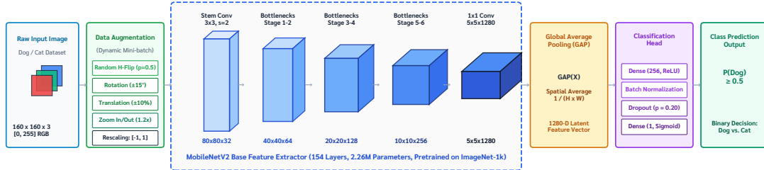
Figure 2(a): End-to-End Transfer Learning Computational & Tensor Pipeline
